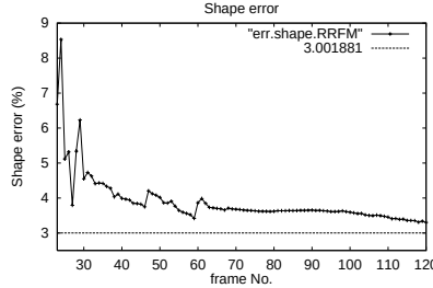
Fig. 2. Shape error.
